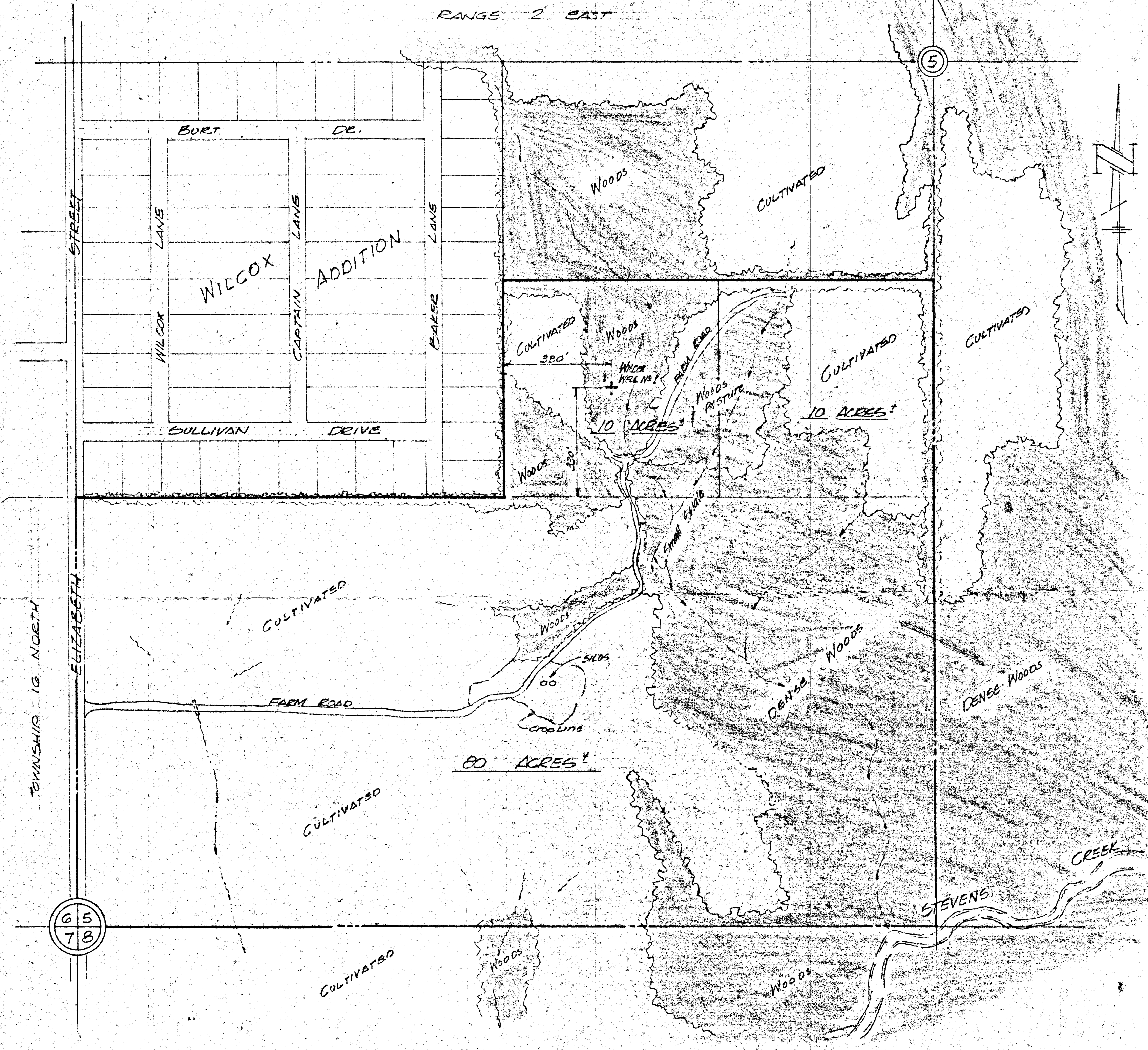
OIL WELL SITE PLAN 1" = 200'
